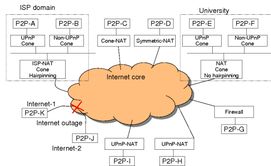
Figure 1: Illustration of the connectivity-constrained wide-area deployment scenario targeted by deployments of the IPOP P2P system.
