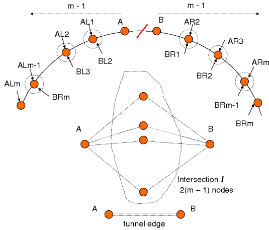
Figure 4: Tunnel edge between nodes A and B that cannot communicate over TCP or UDP transports.
